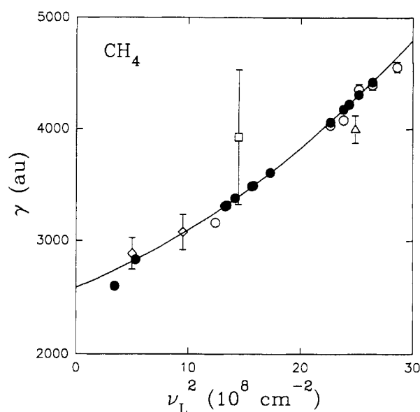
Figure 7. Experimental measurements of \gamma^{vR} for the CH 4 molecule are compared. The solid curve is eq 18 fit to the ESHG data indicated by the filled circles, 34,43 with the \lambda = 1319 nm point excluded from the fit. The true dispersion curve may turn down sharply at low frequency due to \gamma^{vR} , as is suggested by the dispersion curve for \gamma of H 2 in Figure 5, but the frequency dependence of \gamma^{vR} for CH 4 is presently unknown. Other measurements are indicated by open symbols (circles, ESHG; 52,55 triangle, THG; 62 diamonds, dc Kerr; 22,28 square, CARS 73 ). The static SCF result from Table XII, \gamma^e = 1870 au, 227 falls off scale. One expects that \gamma^{vR} versus \nu_L^2 will follow a different dispersion curve for each nonlinear optical process even though \gamma^e versus \nu_L^2 may be described by a single dispersion curve. Comparison of the dispersion curves for \gamma^{vR} would allow one to obtain an experimental estimate of \gamma^{vR} . The present measurements appear to be consistent with a single dispersion curve, which seems to indicate that \gamma^{vR} is small compared to \gamma^e for CH 4 .
